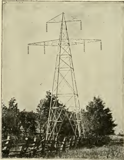
Fig. 178. Modern High-Tension Tower with Suspension Insulators
